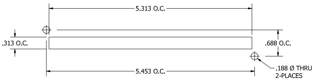
RECOMMENDED MOUNTING HOLE PATTERN
