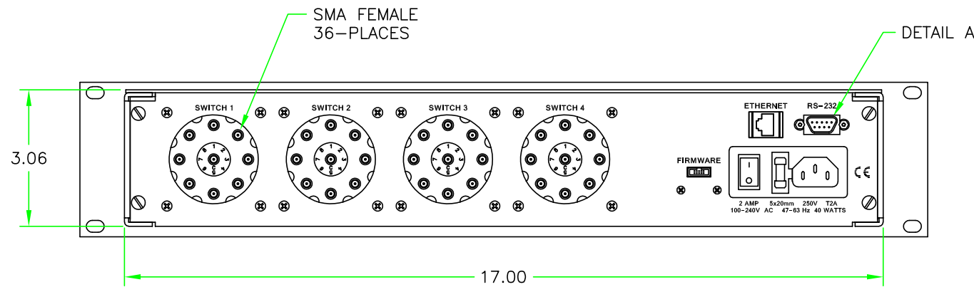
REAR VIEW
