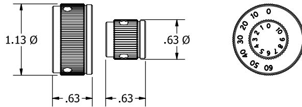
KNOB DETAIL
